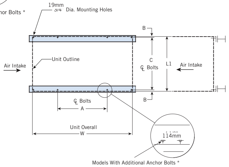
Plan B: Single Cell Unit
