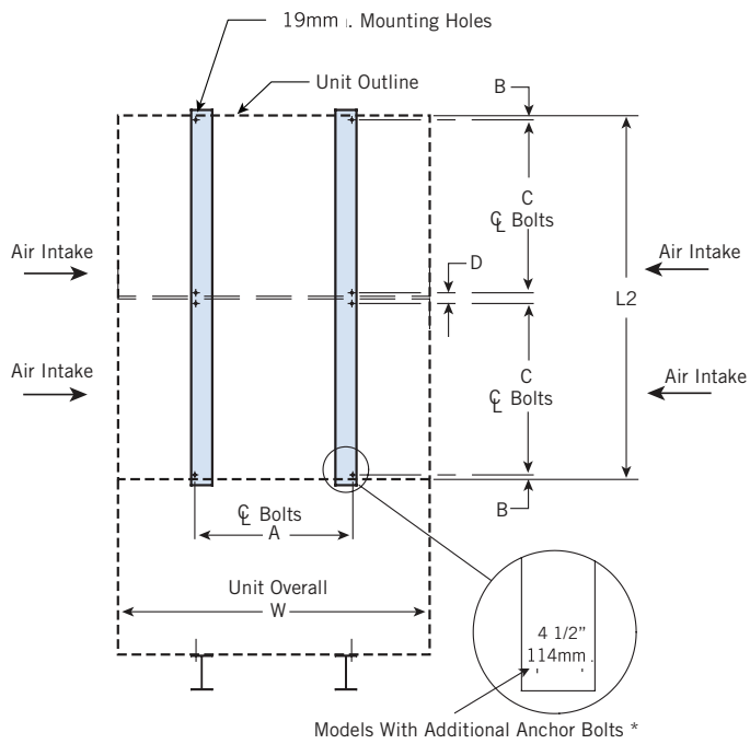
Plan C: Double Cell Unit
