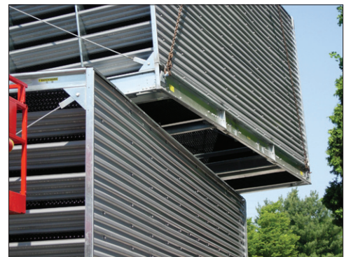
Rigging Guides Ensure Alignment
