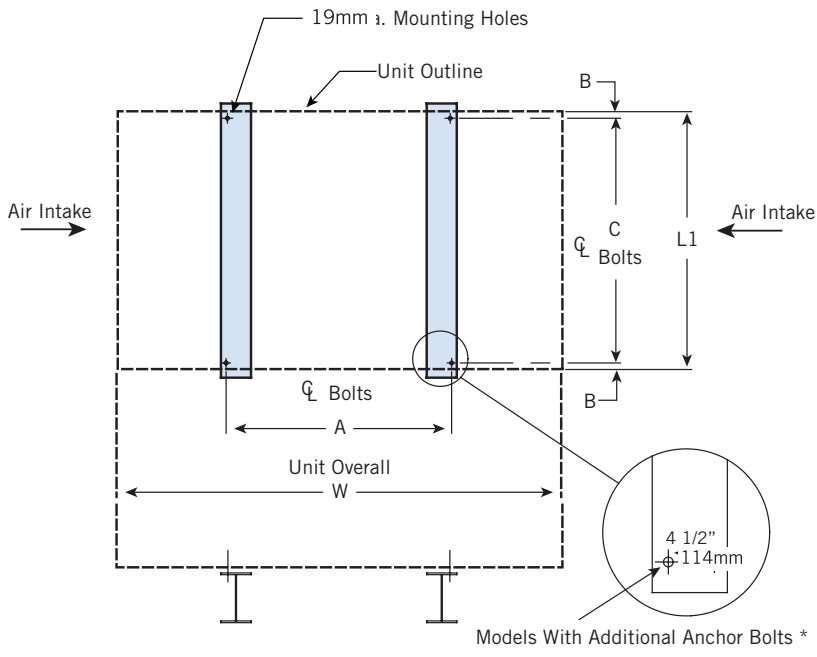
Plan A: Single Cell Unit
